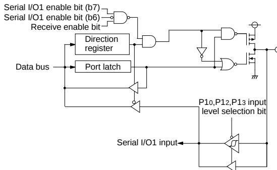
(2) Port P10
